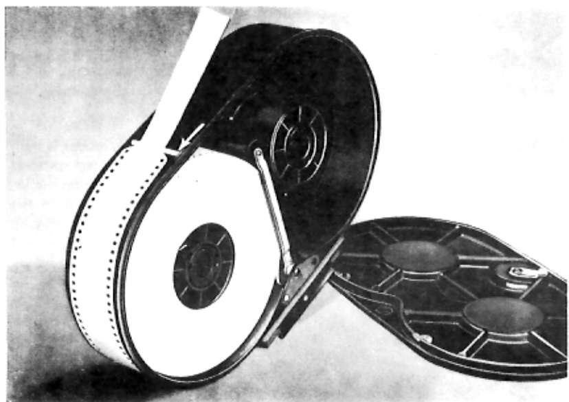
Fig. 5: The film leader is pulled out until the first trimmed holes coincide with the marking rib.
