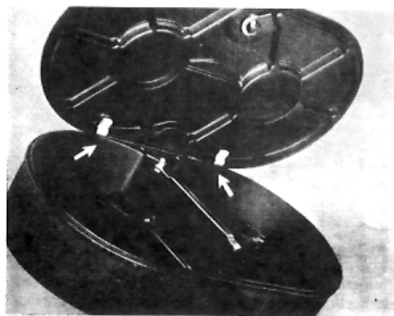
Fig. 7: If the two half hinges are inserted into the slots at the lower rim of the magazine housing correctly, the lid can be shut without the use of force.
