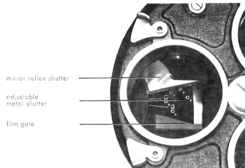
Fig. 14: This for instance is the setting for an aperture of 120.
