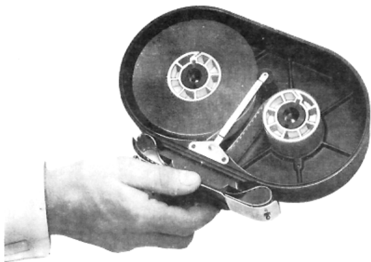
Fig. 8: The film loop guard helps to prevent kinks and other damage to the film.
