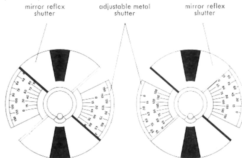
Fig. 13: According to the colour of the edge of the mirror reflex shutter segment visible through the lens socket, the angle of shutter opening can be read off from the outer scale (black) or the inner scale (red).
