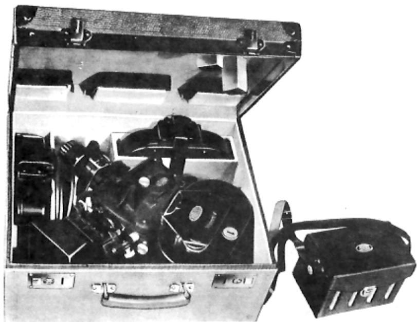
Fig. 16: The small ARRI camera case (Cat. No. 2241) takes an ARRIFLEX 35 II C with mounted 200 ft (60 m) magazine, three spare 200 ft (60 m) magazines together with filters and small accessories and is dust-proof and suitable for use in the tropics.
