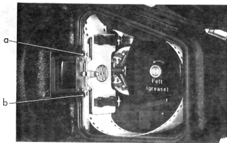
Fig. 10: While threading the film in the camera, make sure that the emulsion side of the film is facing the lens. a and b = film gate fastening strips (see page 26, no. 2).
